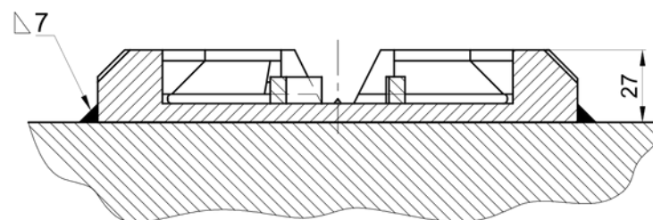
DECK OR HATCH COVER
